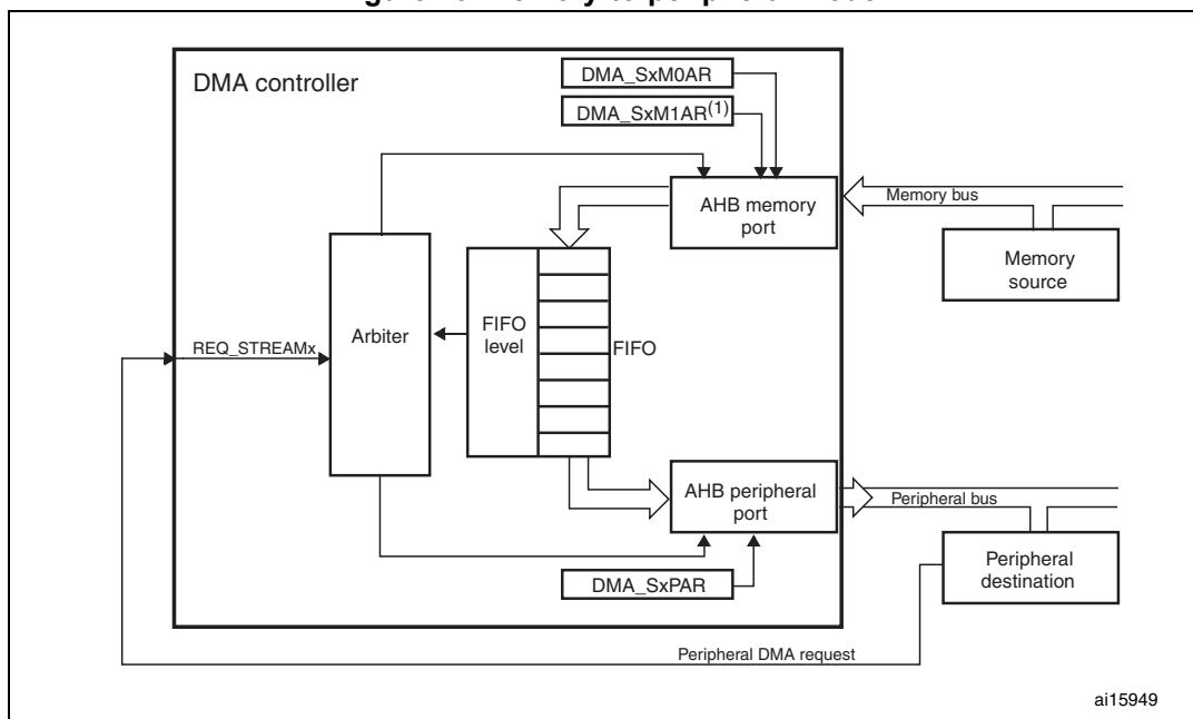
Figure 26. Memory-to-peripheral mode
