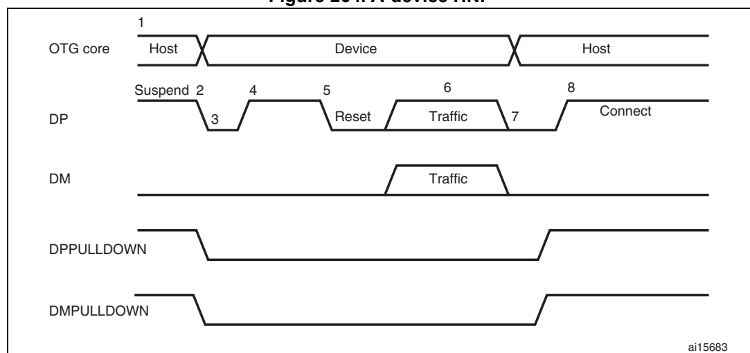
Figure 264. A-device HNP
