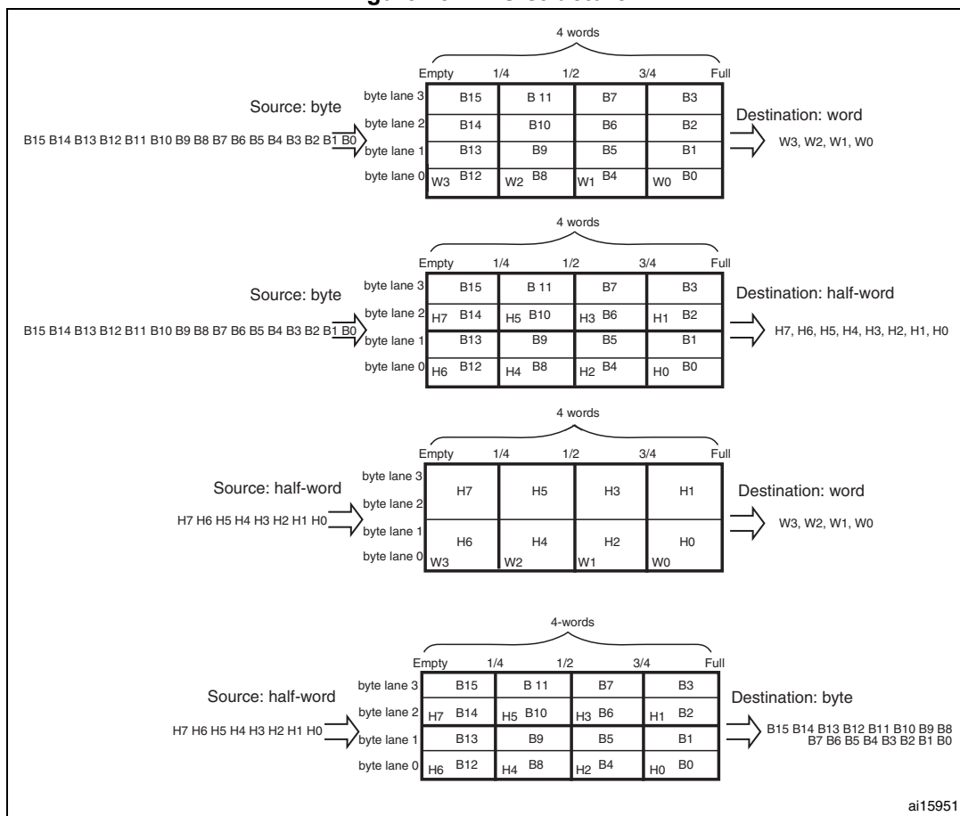
Figure 28. FIFO structure
