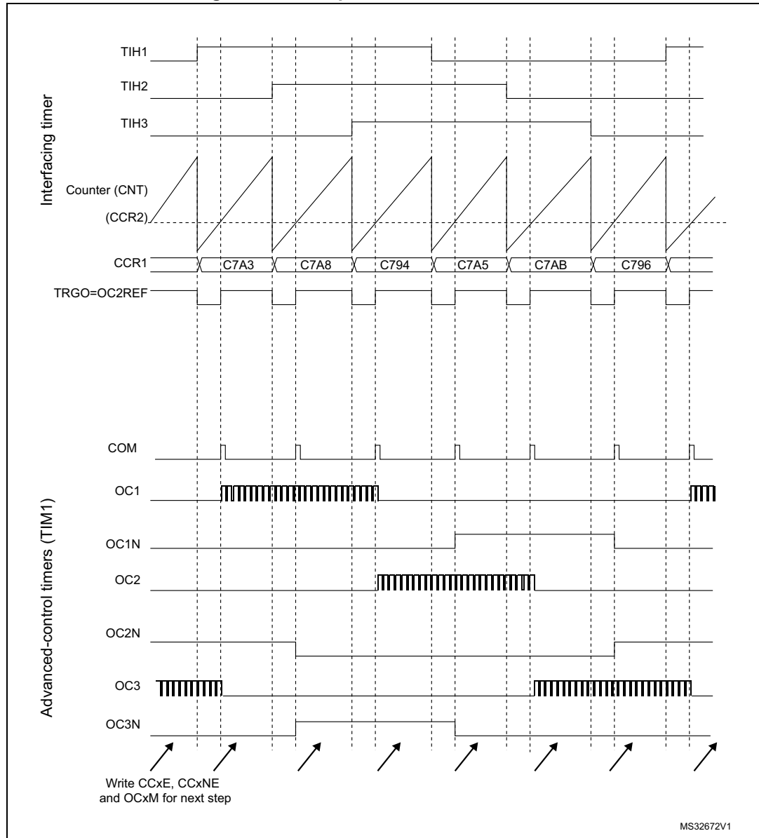
Figure 82. Example of hall sensor interface
