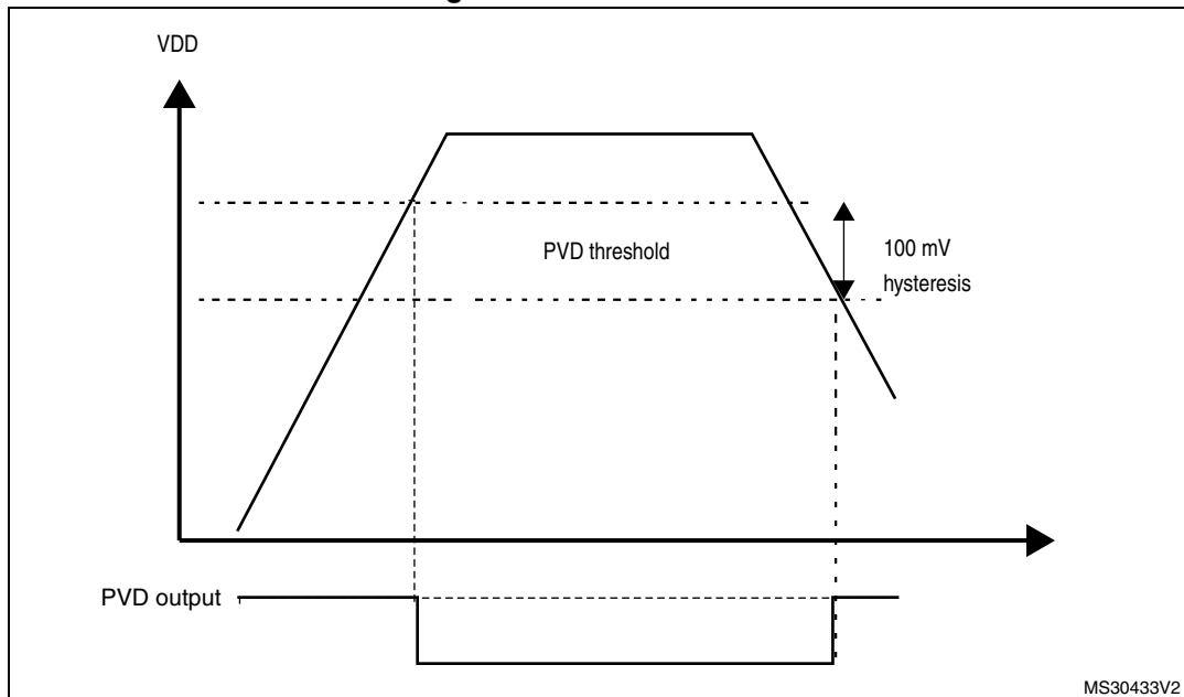
Figure 10. PVD thresholds
