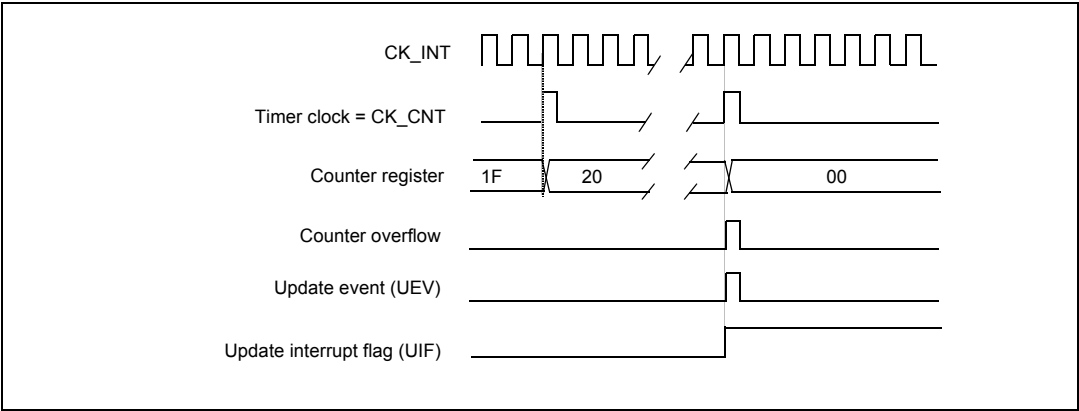
Figure 93. Counter timing diagram, internal clock divided by N
