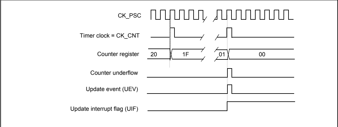
Figure 56. Counter timing diagram, internal clock divided by N
