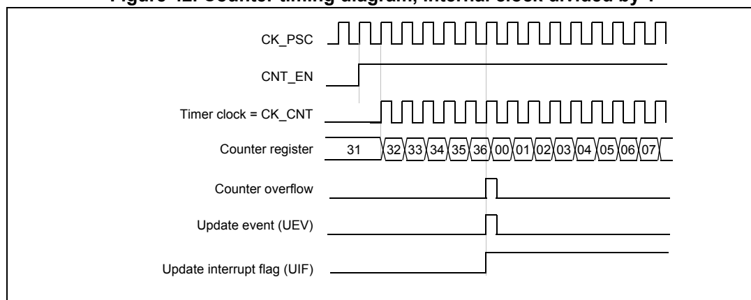
Figure 42. Counter timing diagram, internal clock divided by 1
