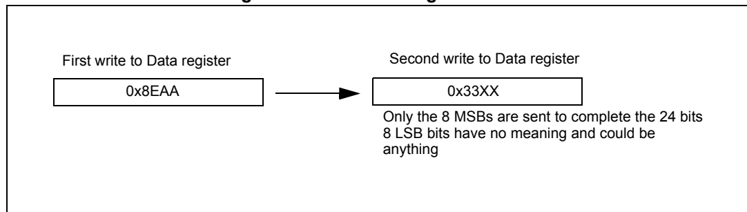
Figure 212. Transmitting 0x8EAA33
